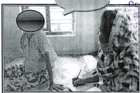
Case Study
